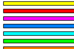
strip.shingle
