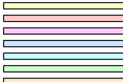
strip.background
