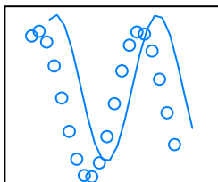
plot.[symbol, line]
