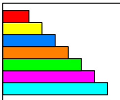
superpose.fill
