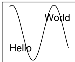
add.[line, text]
