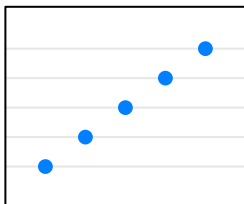
dot.[symbol, line]
