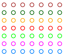
superpose.symbol
